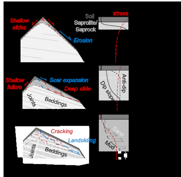
Figure 2, Conceptual schematics illustrating hypothetical mechanisms of cascading mass movements by earthquake (drawn by red) and heavy rainfall (blue) under varying geological conditions (adopted from Matsushi, 2025).
